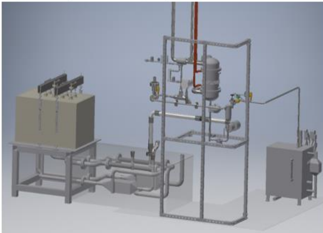
Figure 2. Computer aided drawing of system.
