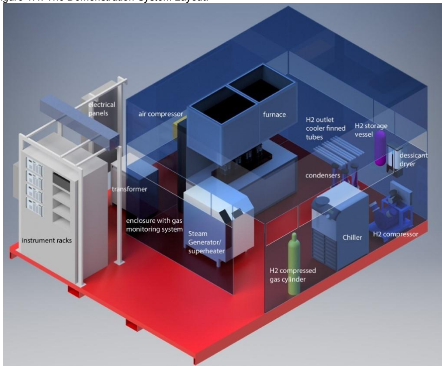
Figure 1.4. The Demonstration System Layout.
