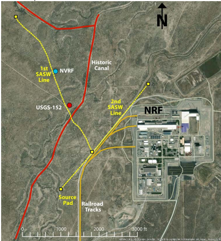
Figure R-2B. USGS-152 seismic velocity borehole (red dot) and NRVF seismic station NVRF (blue dot) near two proposed SASW survey lines (yellow dashed lines) west of NRF.
