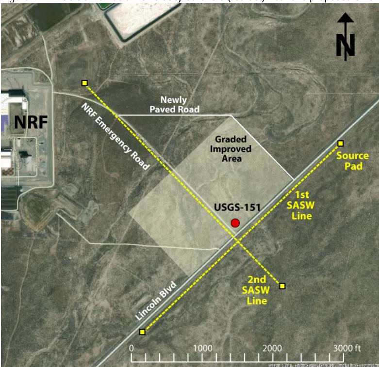
Figure R-2A. USGS-151 seismic velocity borehole (red dot) near two proposed SASW survey lines (yellow dashed lines) east of NRF.
