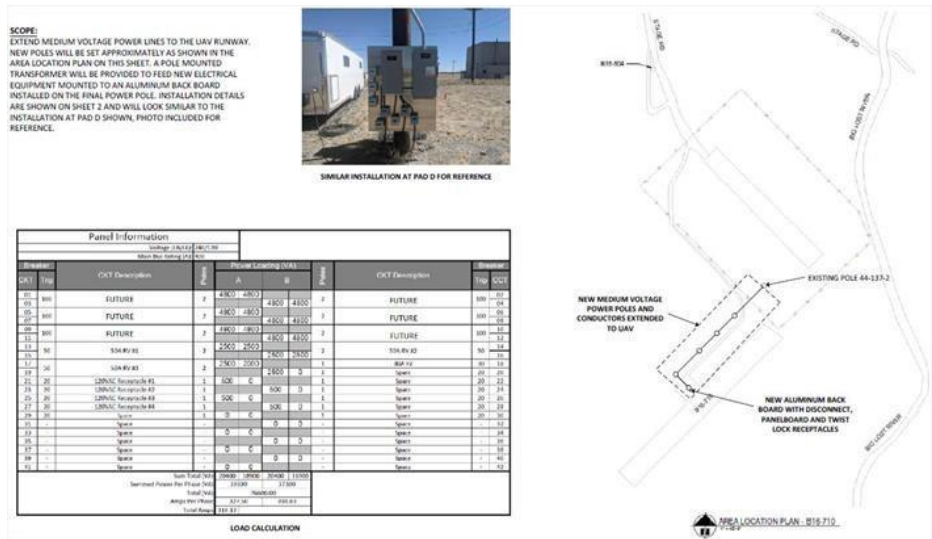
Figure 2-1: Information for electrical upgrade
