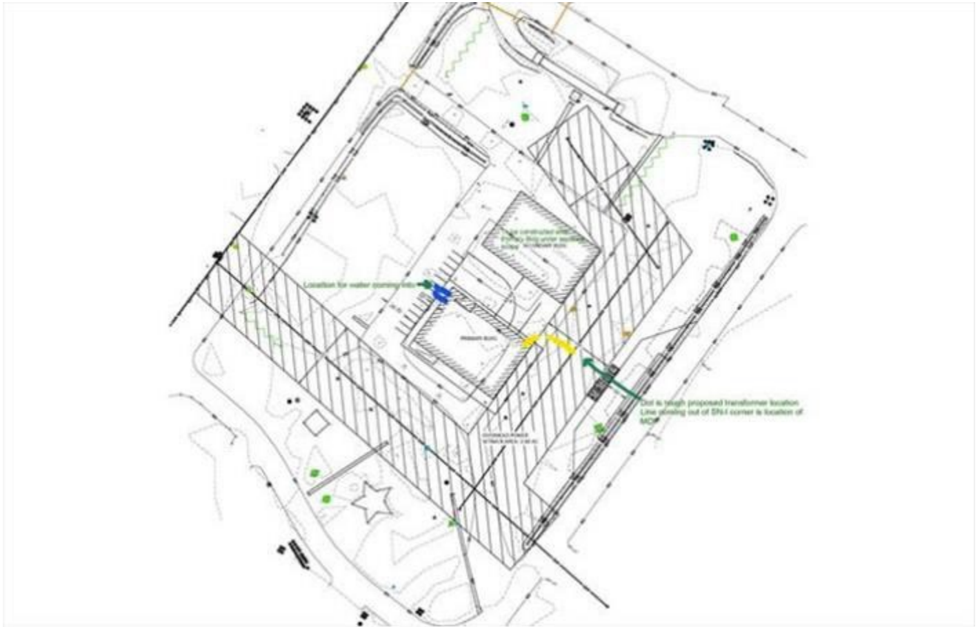
Figure 2. Site plan showing layout building locations and utility tie-in locations. Yellow represents the power connection. Blue indicates the location of the water connection.
